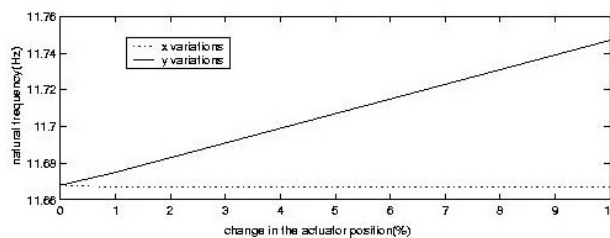
Figure 5. The influences of the actuator placement on the first theoretical natural frequency of the smart beam
