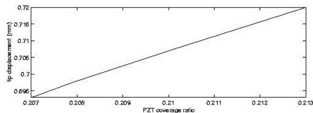
Figure 6. The influence of the actuator size variation on the response of the smart plate
