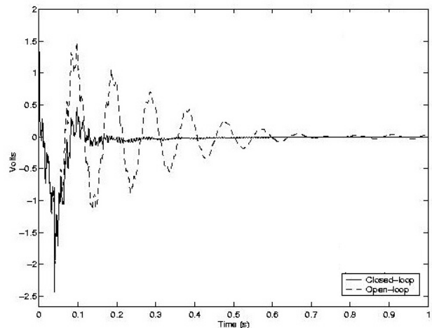
Figure 18. The comparison of the open and closed loop responses to a step input
