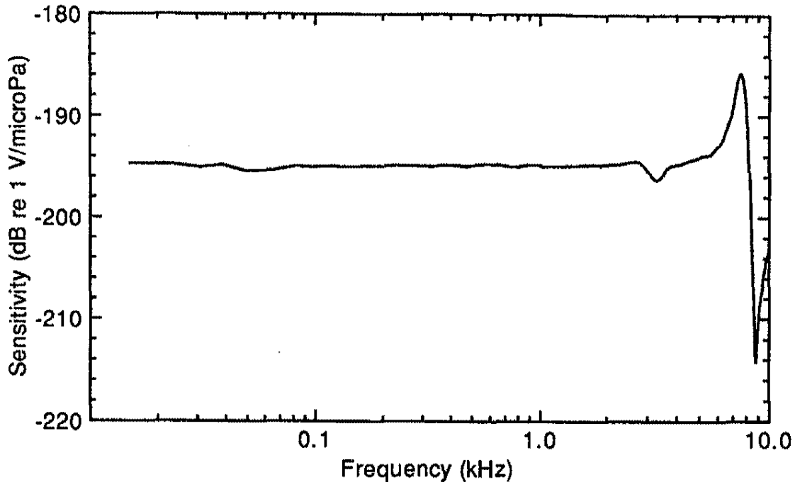
Figure 2: The end-of-cable, free-field, open-circuit voltage sensitivity of the BM024 hydrophone. The frequency ranges from 15 Hz to 10 kHz.
