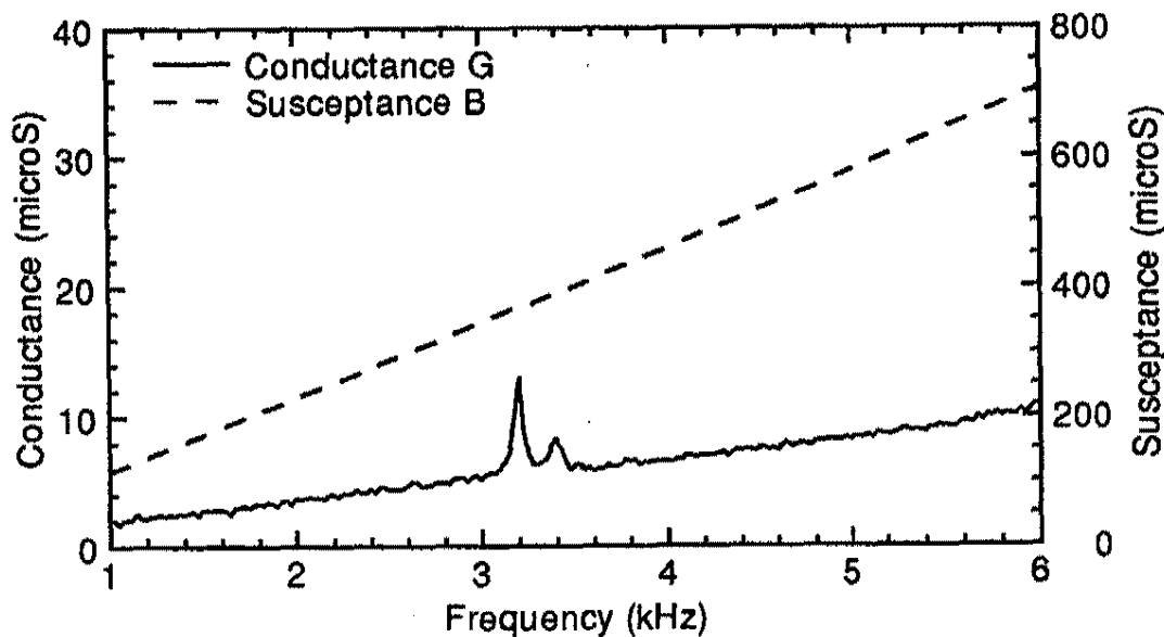
Figure 7: In-air electrical admittance of the BM024 hydrophone over the frequency range 1 to 6 kHz.
