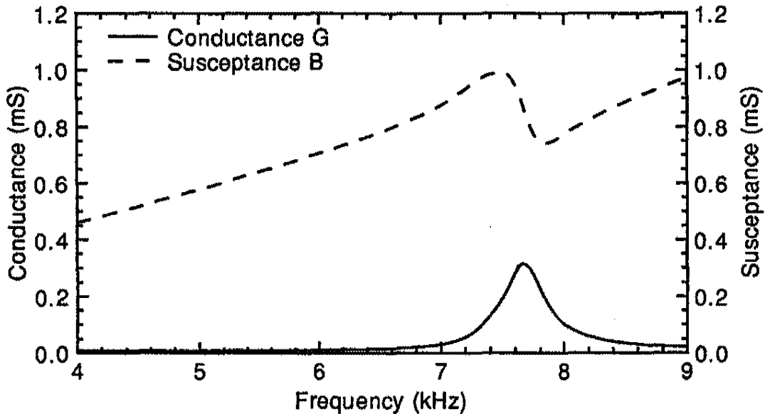
Figure 8: In-air electrical admittance of the BM024 hydrophone over the frequency range 4 to 9 kHz.
