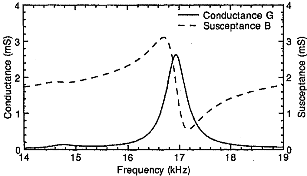
Figure 9: In-air electrical admittance of the BM024 hydrophone over the frequency range 14 to 19 kHz.
