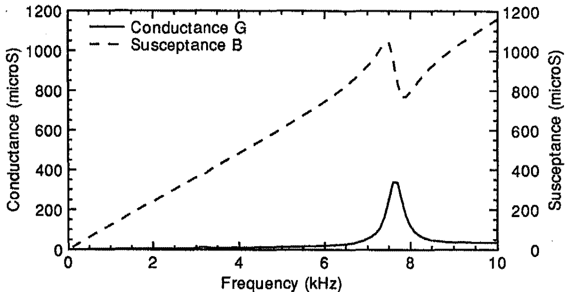
Figure 4: In-water electrical admittance of the BM024 hydrophone, measured at the end of a 3.9 m cable.
