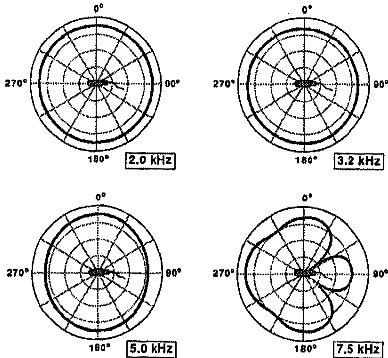
Figure 6: Directivity patterns of the BM024 hydrophone in the XZ plane. The scale, from the center to the top of the grid in each pattern, is 40 dB.
