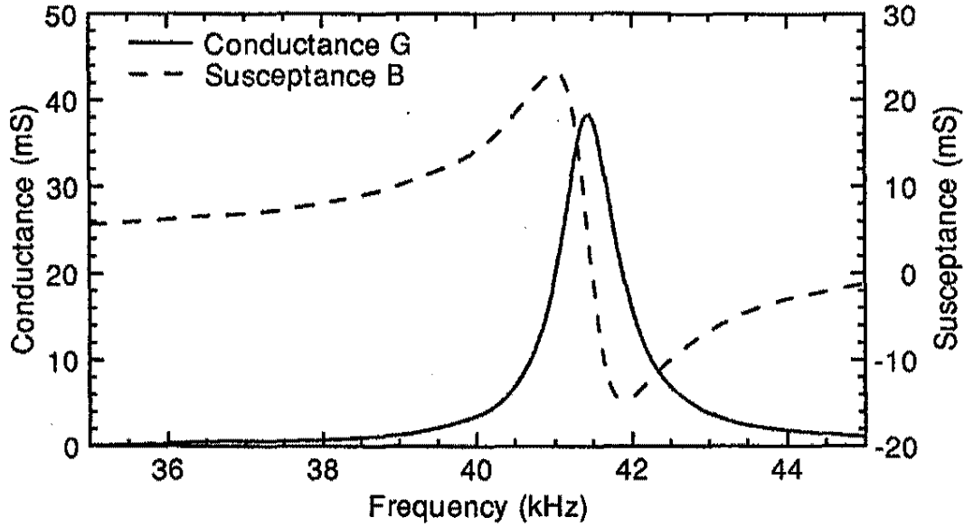
Figure 10: In-air electrical admittance of the BM024 hydrophone over the frequency range 35 to 45 kHz.
