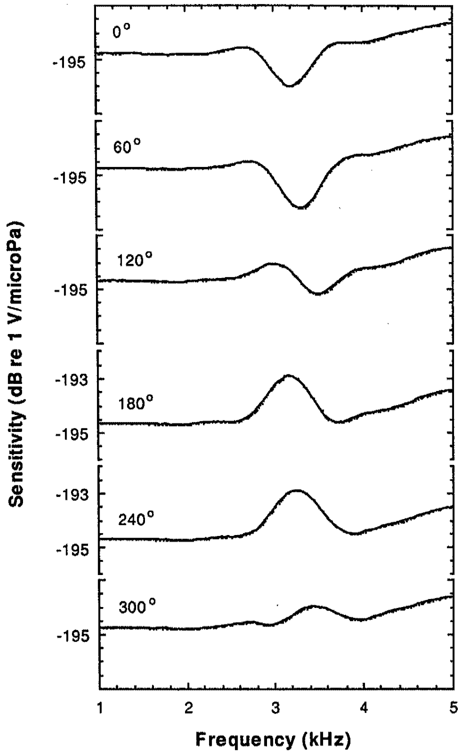
Figure 3: The sensitivity of the BM024 hydrophone as a function of the angle to the source, for the frequency range 1 to 5 kHz. Each vertical axis is 10 dB.
