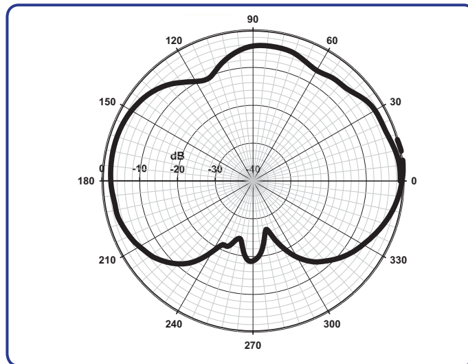
Directivity Pattern at 30 kHz, Axial Plane
