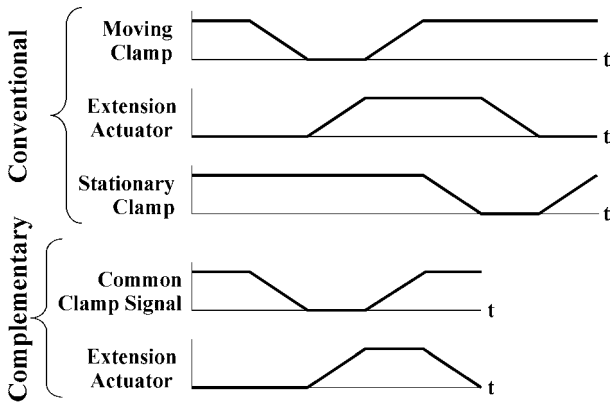
Fig. 3. Inchworm actuator conventional and complementary drive signals.
